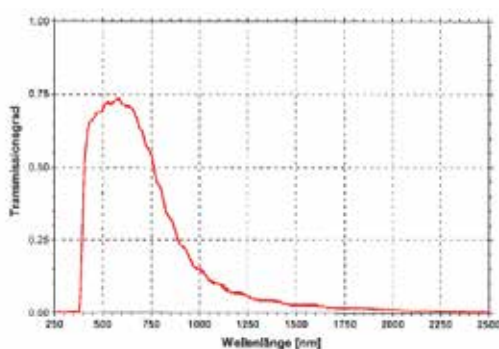
Transmissionsgrad ARCtec-TR 70
